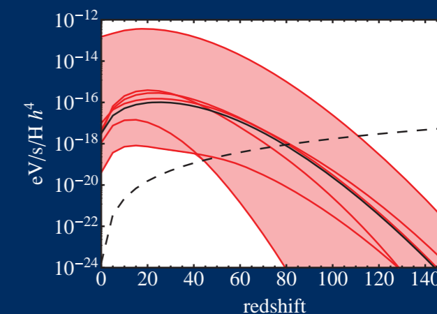
A plot of mean power output per hydrogen nucleus from the annihilation of Dark Matter as a function of redshift. The black solid line is the fiducial model from Mack’s paper, with other possible models represented by the red solid lines. The black dashed line corresponds to annihilation from the smooth component. The red shading represents the range of annihilation power predictions corresponding to the models considered in the analysis.
