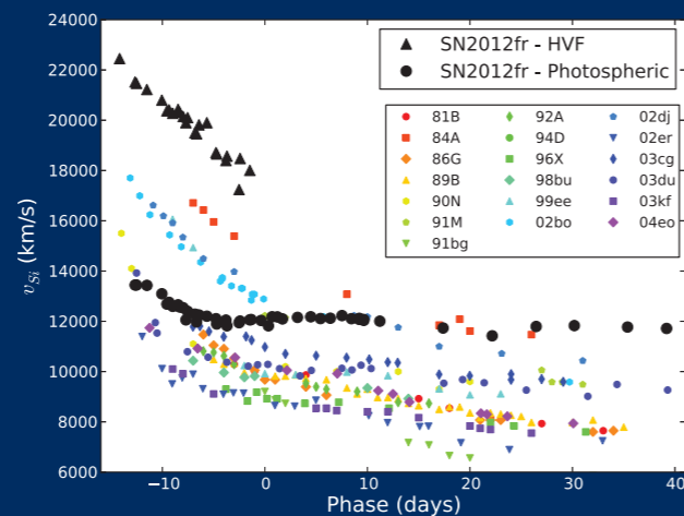
The velocity evolution of the Si II \lambda 6355 feature of Supernova 2012fr compared to that of a number of type Ia supernovae from a previous sample. The high-velocity feature component of SN 2012fr is shown as large black triangles, while the lower velocity photospheric component is shown as large black circles.
