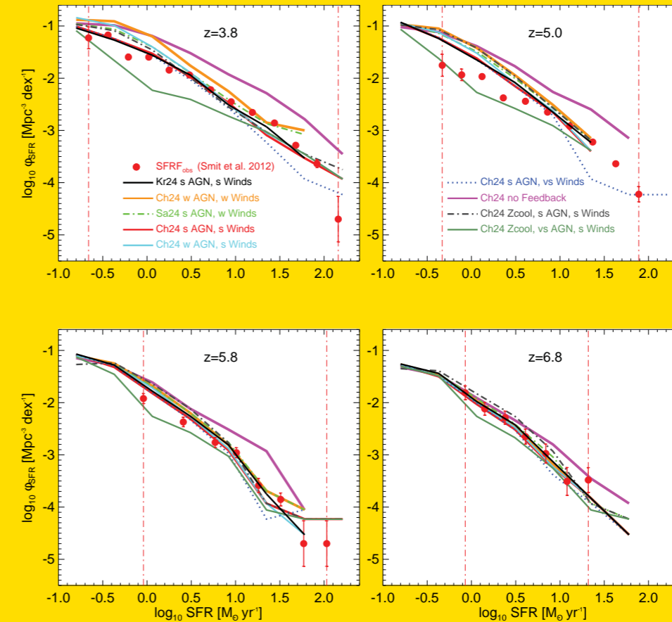
A plot of the simulated star formation rate functions at z \sim 4 - 7 , compared to recent observational results (Smit et al. 2012).
