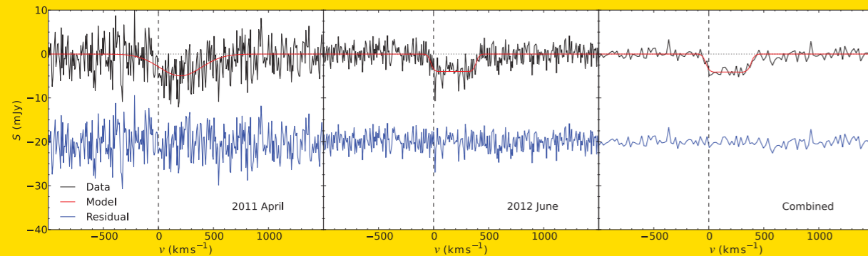
The results of fitting HI absorption to spectral data taken in April 2011 and June 2012 with the Australia Telescope Compact Array. The black line represents the data after subtracting the best-fitting (i.e., maximum likelihood) continuum component, and the red line represents the best-fitting spectral line model. The blue line is the resulting residual.
