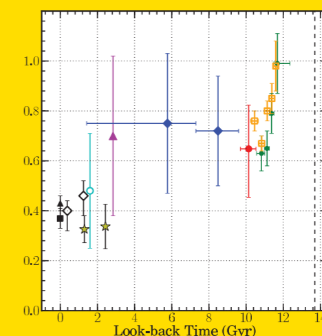
The evolution of the cosmic neutral hydrogen gas density over time. Rhee et al.'s observations are represented by the gold stars and show no change between z = 0 and z = 0.2 . This is in stark contrast to the substantial evolution seen to be occurring at earlier times.
