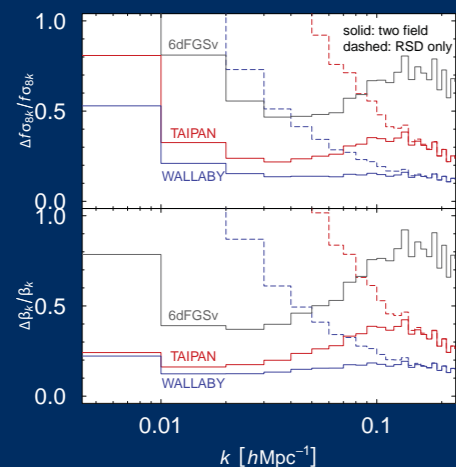
Predicted constraints on cosmological parameters f\sigma_8 and \beta for different data sets. The plots show how redshift surveys constrain the linear growth rate, amplitude of matter perturbations and galaxy bias as a function of inverse scale, k , for the 6dF Galaxy Survey velocity subsample (6dFGSv, grey line), the TAIPAN survey (red lines), and for the combination of the WALLABY and WNSHS 21cm radio surveys (blue lines). Dashed lines are for redshift samples, and solid lines are for peculiar velocity subsamples. Peculiar velocity surveys improve the constraints for k < 0.1 , because they are not limited by the cosmic variance.
