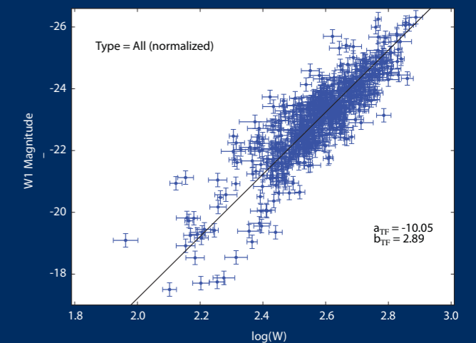
The WISE mid-infrared Tully-Fisher relation after all the galaxies in the sample have been normalised to an Sc/Sd morphology.
