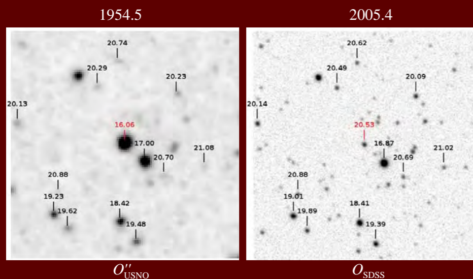
These two images, one from 1954 and the other from 2005, show a previously unknown variable star. Recalibrated magnitudes are shown in each image. The object labelled in red has decreased in brightness by 4.5 magnitudes between the observations. The extent of the object's change in brightness, its extremely red colour and its high infrared brightness all suggest that it is a Mira variable.
