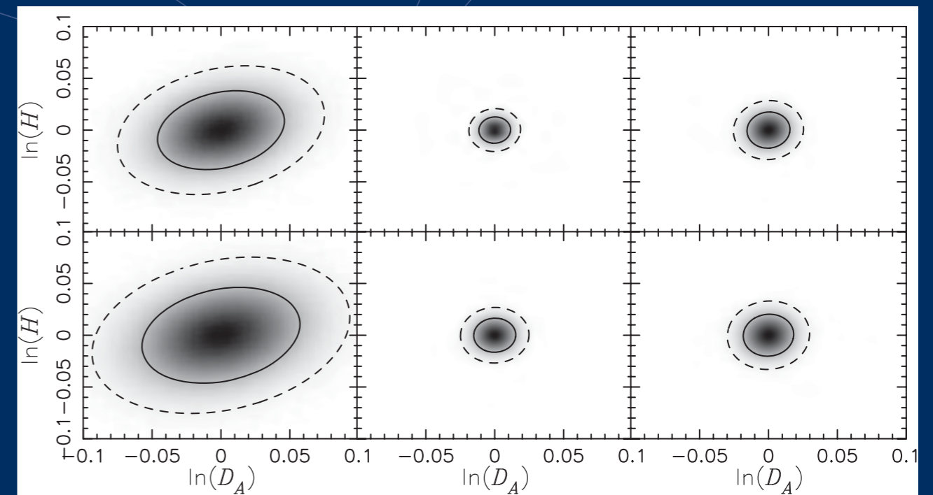
Two-dimensional likelihood distributions for the angular diameter distance, D_A , and the Hubble rate, H , predicted for HETDEX, with 1\sigma and 2\sigma likelihoods shown as solid and dashed contours, respectively. From left to right, the columns show the constraints generated only from the Lyman-alpha galaxy reduced bispectrum, from the Lyman-alpha galaxy power spectrum and bispectrum combined, and from the Lyman-alpha galaxy power spectrum and reduced bispectrum combined. The top row shows the fiducial case with no Lyman-alpha radiative transfer effects included, while the bottom row shows the improvement produced when including first-order Lyman-alpha radiative transfer effects.
