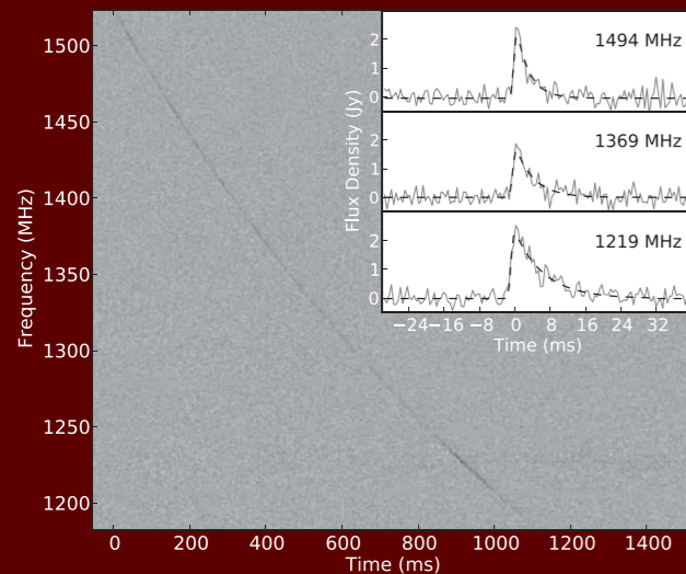
A greyscale of fast radio burst FRB 110220, the brightest burst detected with the Parkes radio telescope, showing the characteristic frequency-dependent delay expected. In the inset, the pulse profile is shown as a function of frequency for various sub-bands, demonstrating the expected increase in pulse width due to scattering in intervening gas.
