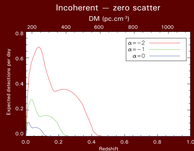
The expected number of detections per day per z = 0.01 redshift bin for the Murchison Widefield Array, using an incoherent combination of signals from each of the 128 tiles. Rates are shown for three values of the source spectral index \alpha .
