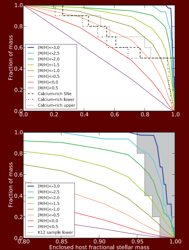
The observed distribution of peculiar supernovae within galaxies, compared to those of stars of different metallicity and older than 10 billion years, as predicted by the team's simulation. The full sample of supernovae studied is in the top panel. In the bottom panel, the shaded area represents the contour for the five best-studied supernovae in the sample.
